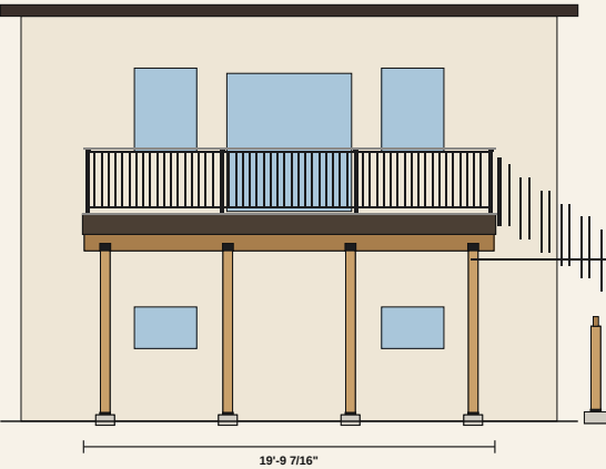
FRONT ELEVATION — from the yard
