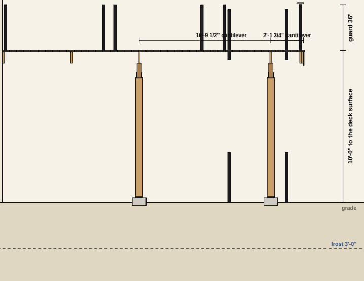
SECTION through zone A at 9'-10 3/4" — looking toward the left end
